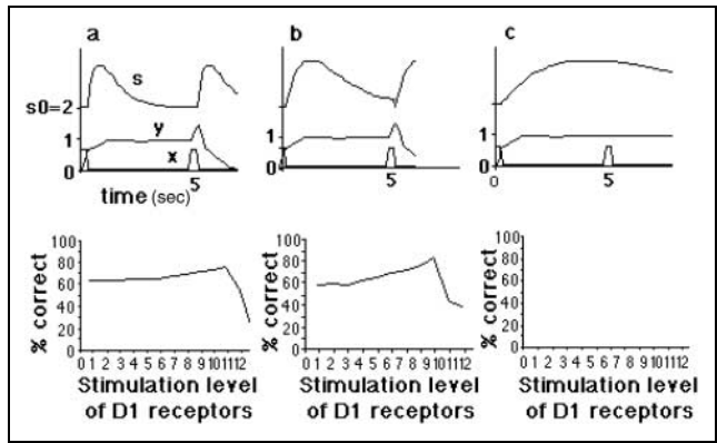
Figure 4. Top: Time course of the network activity y and of the postsynaptic effect of dopamine (temporary threshold s ) in the PFC for two successive transitory excitatory inputs x when the time constant of the threshold is lower (case a), adapted (case b) or higher (case c) than the delay. Bottom: Network performance for increasing level of D1 receptors stimulation in cases a, b, and c. Noise is distributed according to a Poisson process of mean 5 sec.
